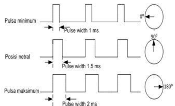
Gambar 4. Pulse Wide Modulation
