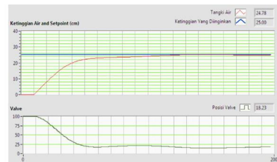
Gambar 15. Hasil percobaan PID ideal tipe PI
