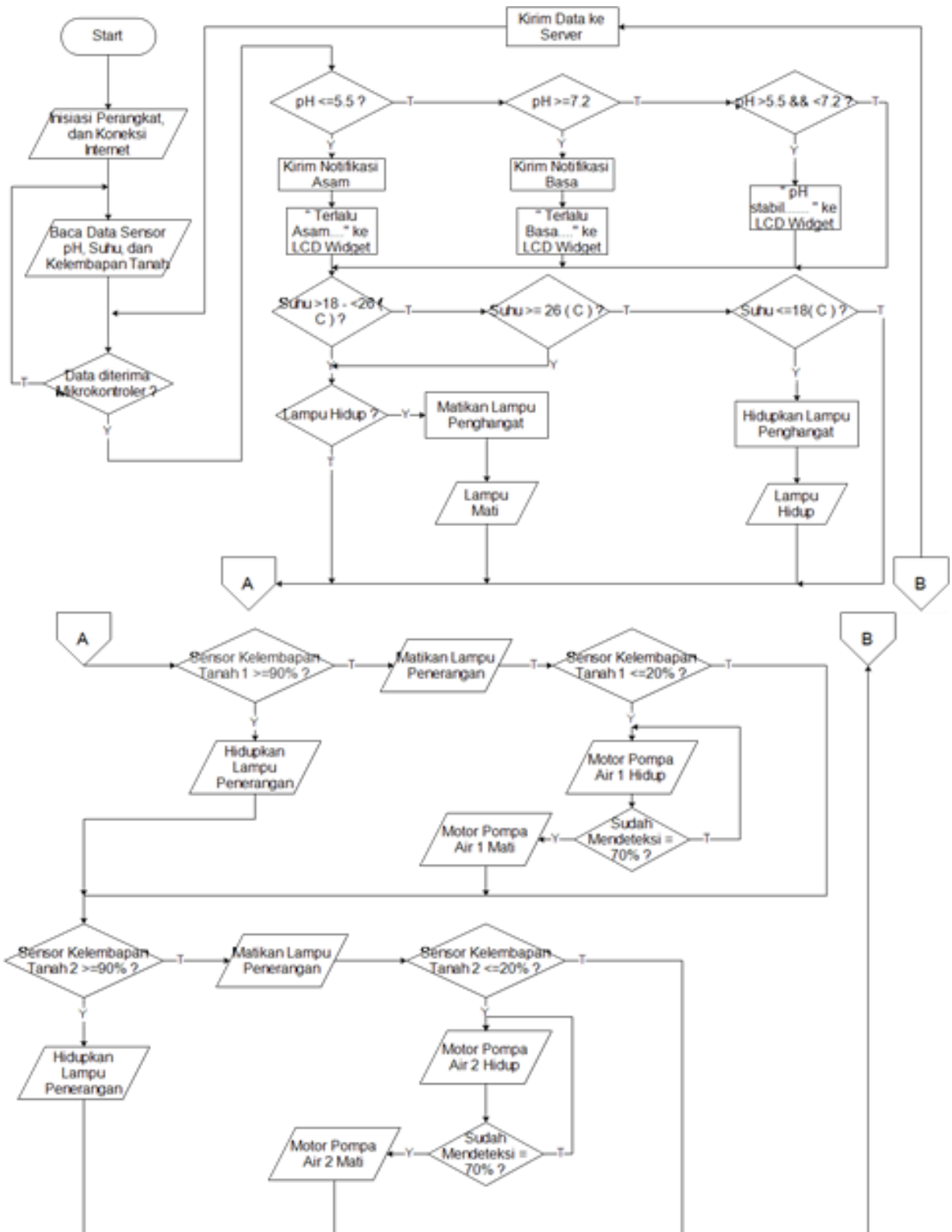
Gambar 9. Flowchart Sistem
