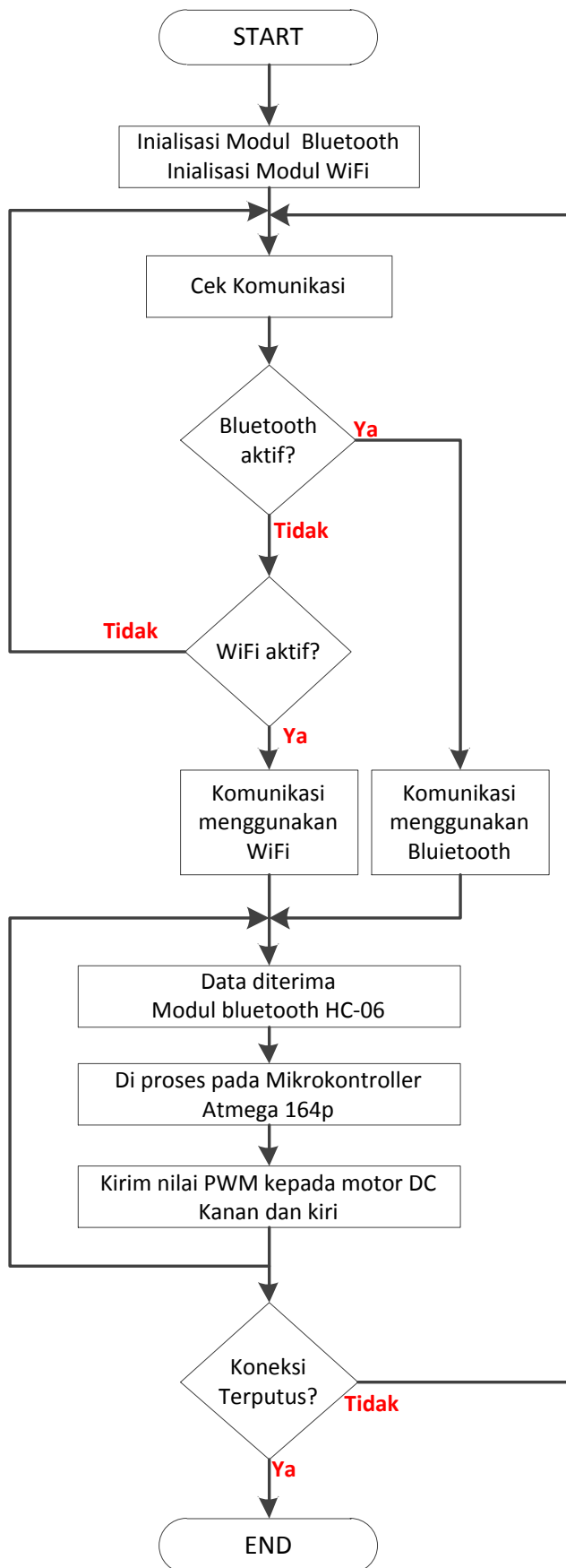
Gambar 10. Diagram Alur (flowchart) Robot Mobil
