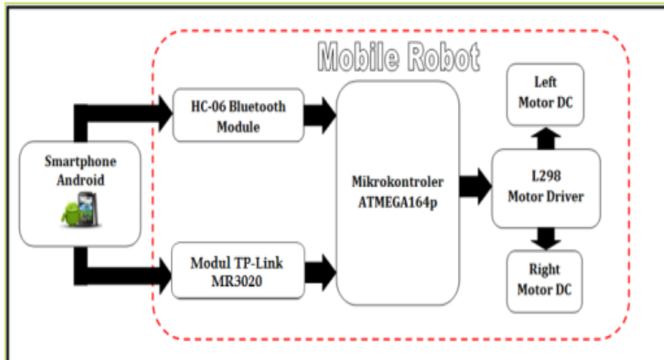
Gambar 2. Block Diagram Sistem
