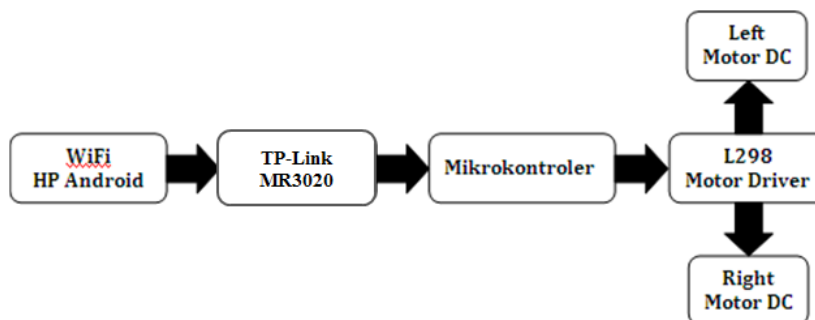
Gambar 8. Diagram Blok Pengontrolan Robot Mobil Via WiFi
