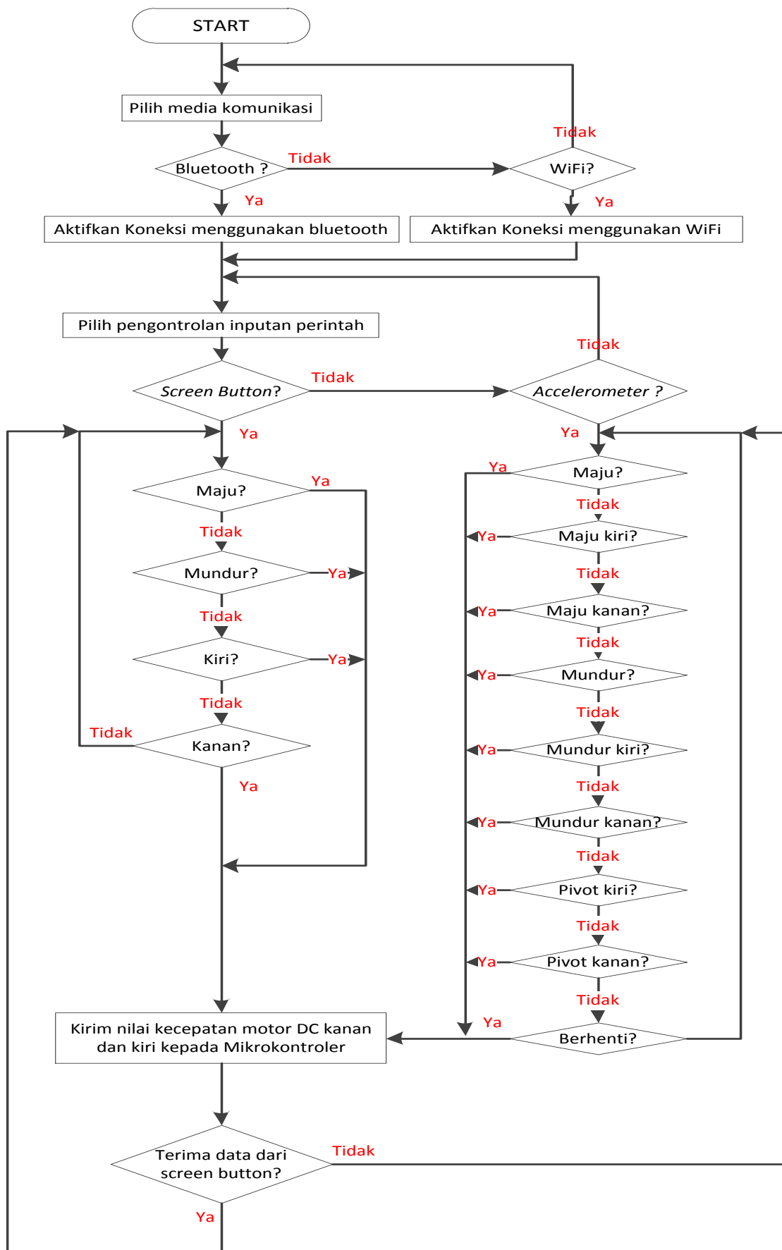
Gambar 11. Diagram Alur (flowchart) Android
