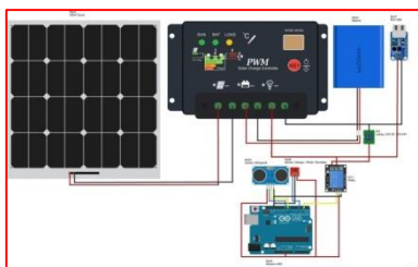
Gambar 11. Rancangan Alat Smart Lighting LED
