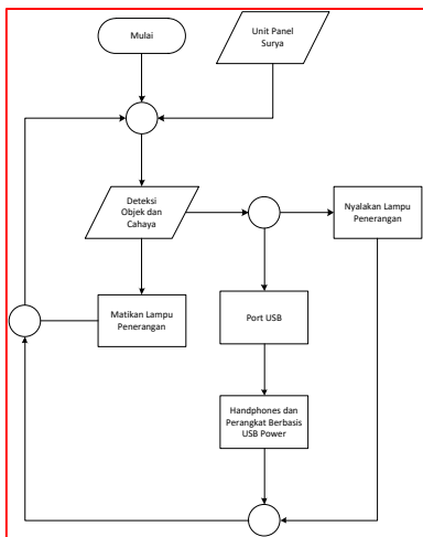
Gambar 10. Diagram Alir Smart Lighting LED
