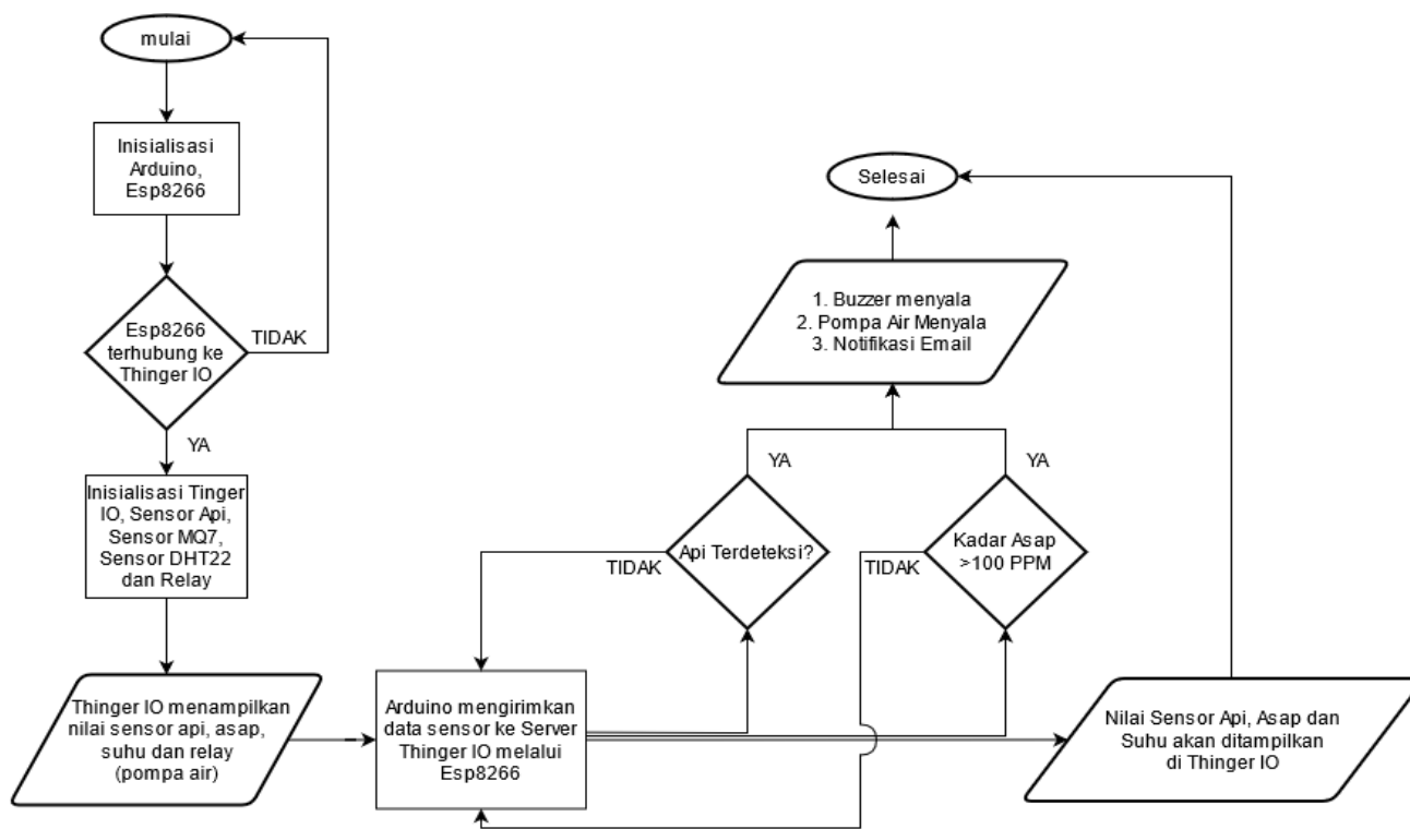
Gambar 2. Flowchart Sistem
