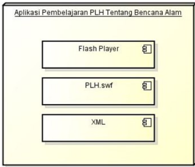
Gambar 18. Diagram Deployment
