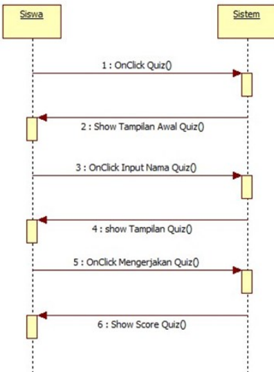
Gambar 11. Sequence Diagram Quiz
