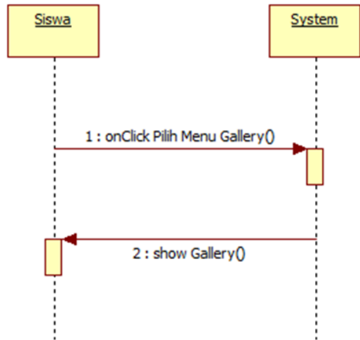
Gambar 16. Sequence Diagram Gallery
