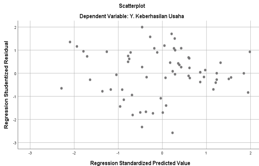
Gambar 1 Scatterplot Uji Heteroskedasiditas
