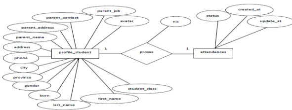
Gambar 6. Entity Relationship Diagram
