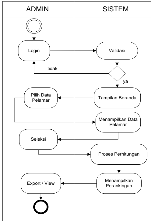
Gambar 6. Activity diagram seleksi
