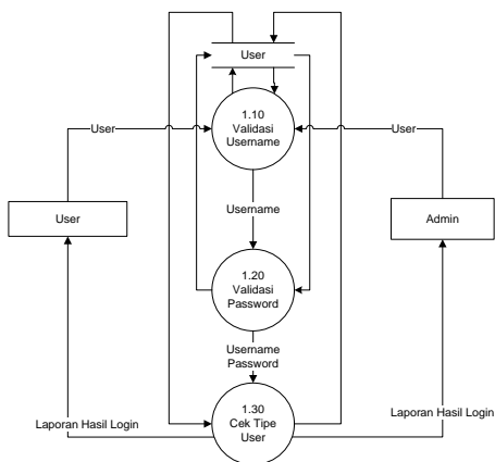
Gambar 4.4 DFD Level 1 Proses 1.00 Login
