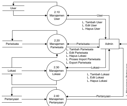
Gambar 4.5 DFD Level 2 Proses 2.00 Master
