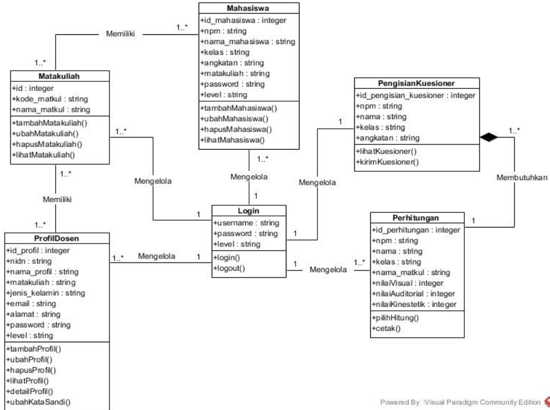
Gambar 4. Class Diagram
