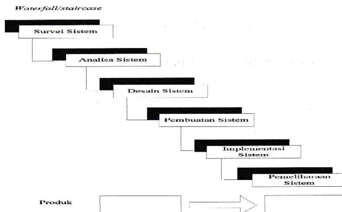
Gambar 1 Waterfall (Sutabri, 2004:63)
