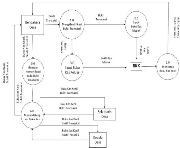
Gambar 7 Data Flow Diagram
