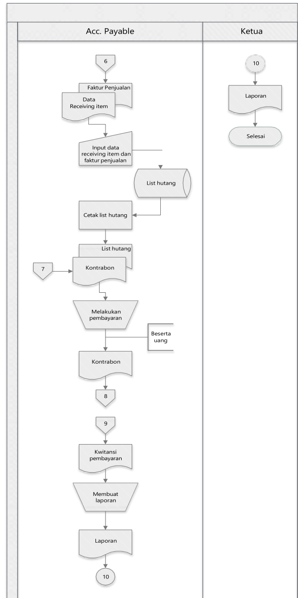
Gambar 4. Flowchart sistem(3)
