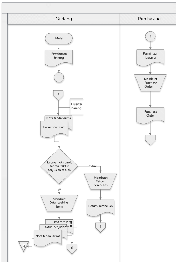
Gambar 2. Flowchart sistem (1)
