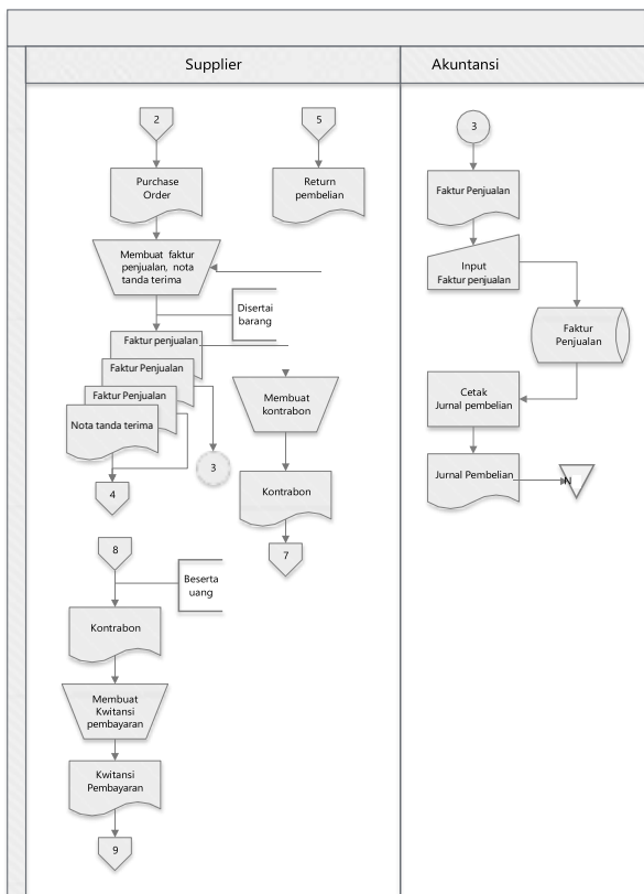
Gambar 3. Flowchart sistem (2)
