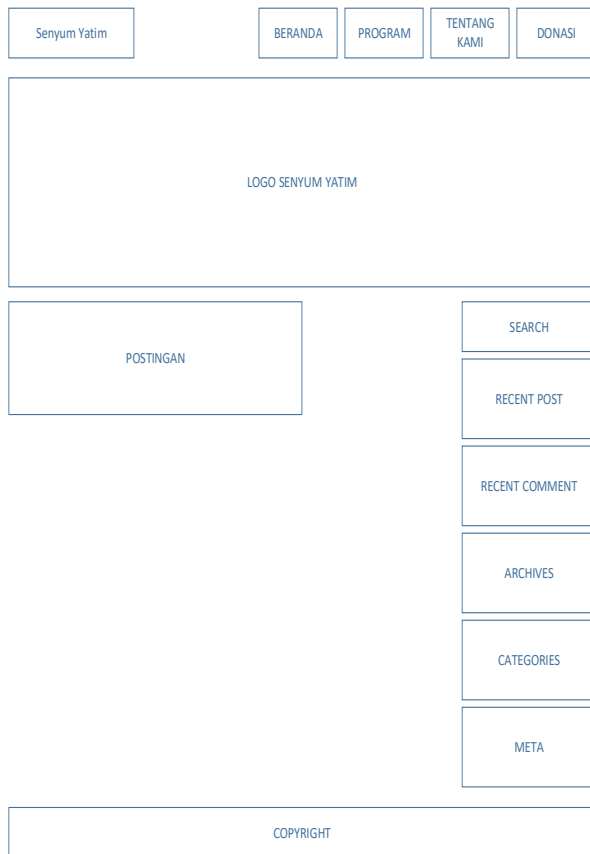
Gambar 1.2 Layout Web
